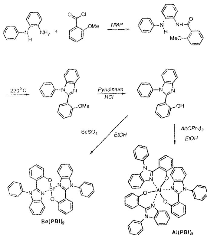
Scheme 1. Synthesis of Al(PBI) 3 and Be(PBI) 2 .
