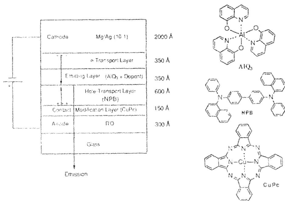
Fig. 1. Multilayer structure of a thin-film EL device.
