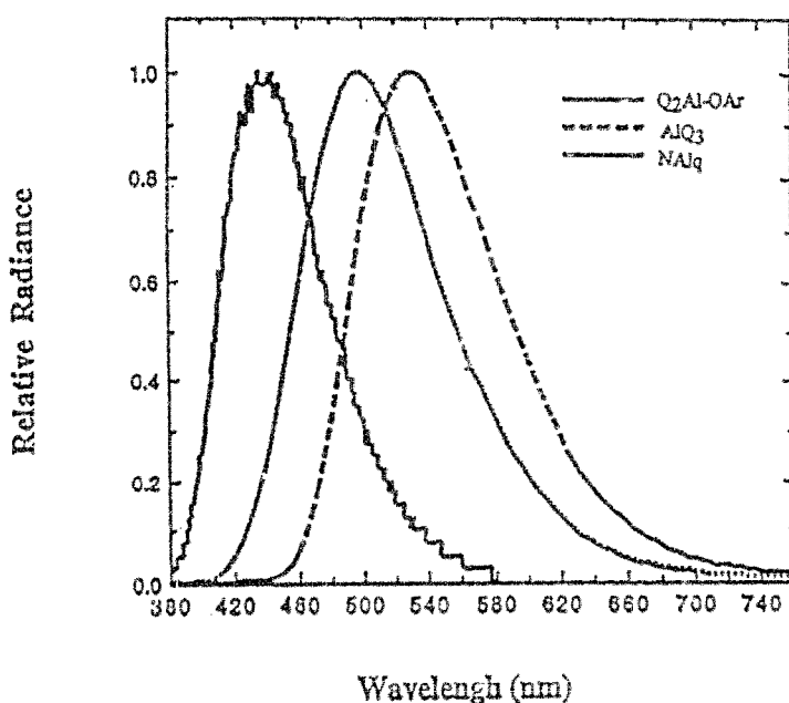
Fig. 3. Photoluminescence spectra of \text{Al}(\text{NQ})_3 , \text{AlQ}_3 , and \text{Q}_2\text{Al-OAr} .
